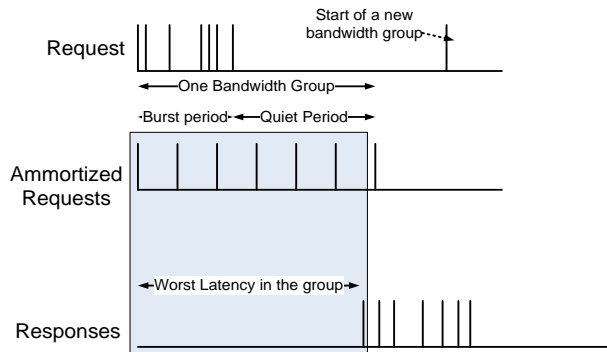
Figure 5: Jitter Measurement
